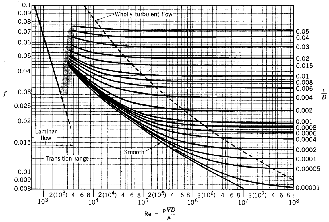
Fig. 4 - Moody Chart (reprinted with permission from Munson et al. 1990)
