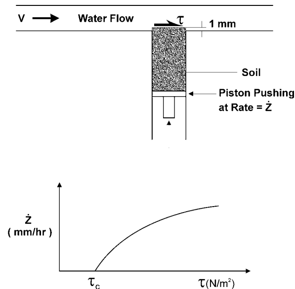
Fig. 1 - Schematic Diagram and Result of the EFA (Erosion Function Apparatus)
