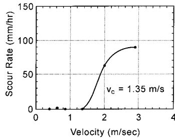
Fig. 3 - Erosion Function for a soil sample taken near Pier 27E of the Existing Woodrow Wilson Bridge (2.6 - 3.2 meters depth) : a) Scour Rate vs. Shear Stress, b) Scour Rate vs. Velocity
