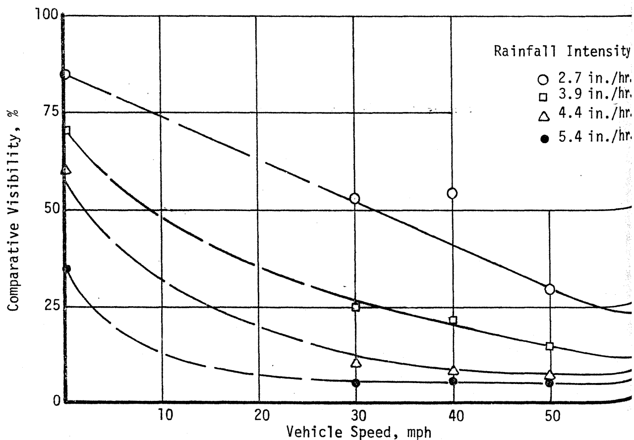
FIGURE 4. PHOTOGRAPHIC ESTIMATE OF VISIBILITY vs. VEHICLE SPEED
