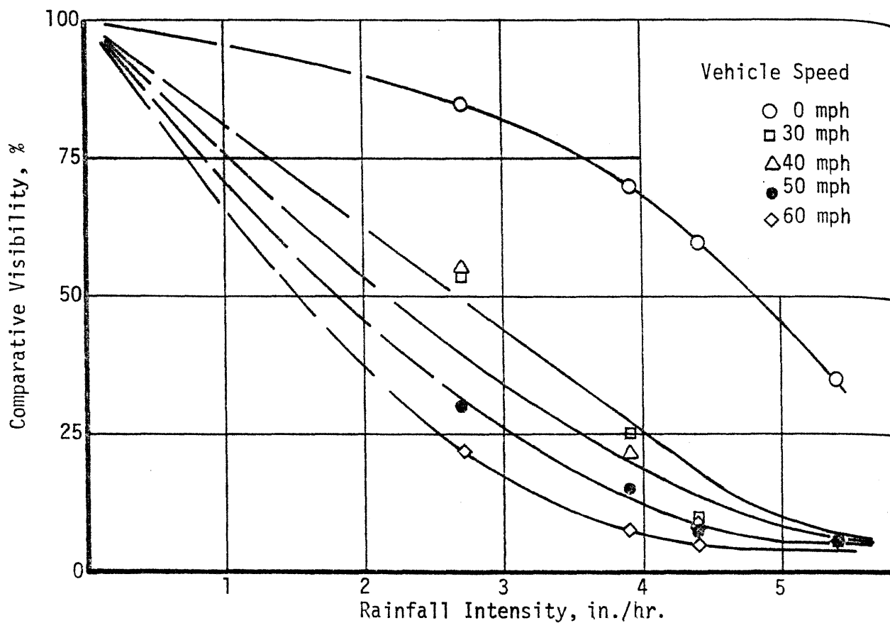
FIGURE 3. PHOTOGRAPHIC ESTIMATE OF VISIBILITY vs. RAINFALL INTENSITY
