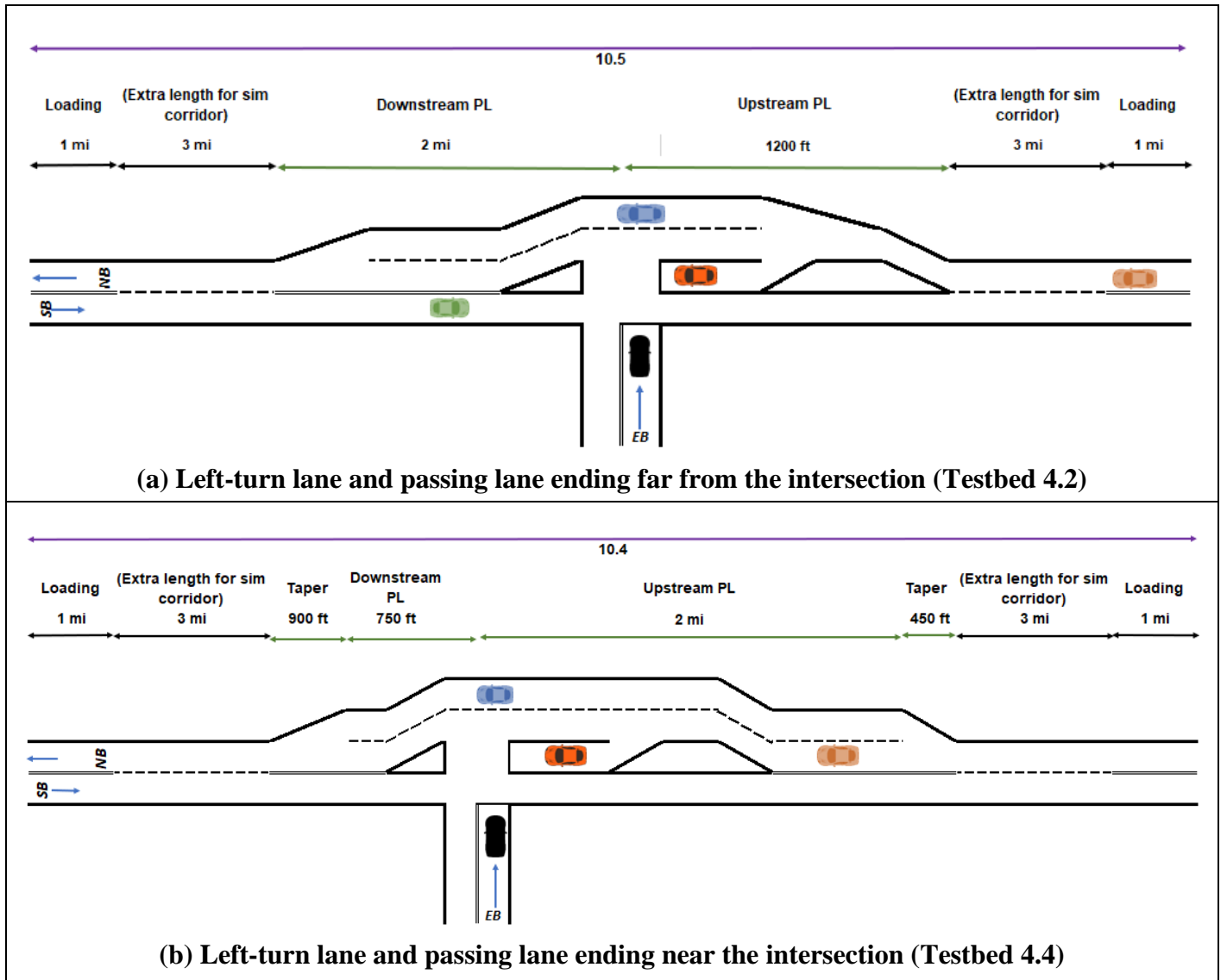
Figure 19. Examples of 4.0 Series Testbeds—Intersections with a Left-Turn Lane within a Passing Lane with Varying Distances to the Start and End of the Passing Lane.
