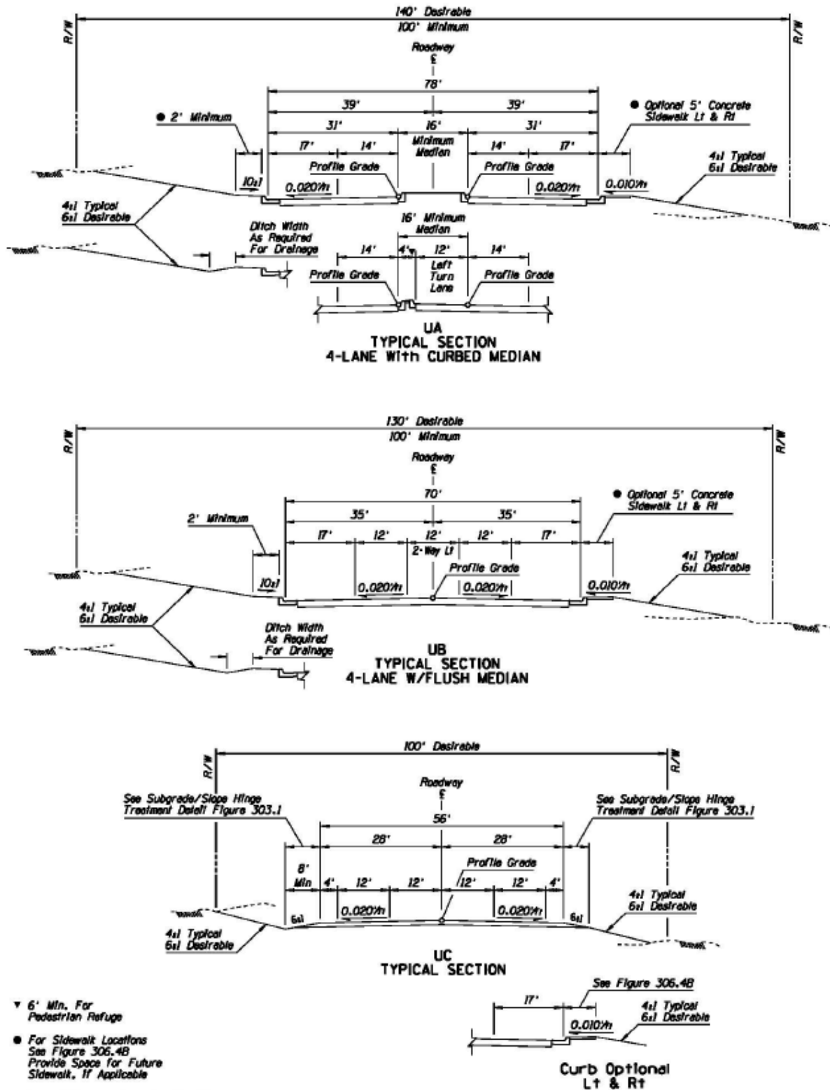
Figure 15. Arizona Urban Highway Typical Sections (Figure 306.4A in 55)
