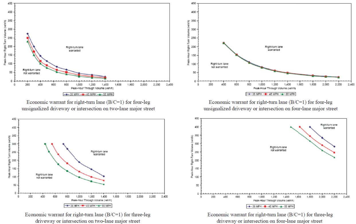
Figure 23. Economic Warrants for Right-Turn Lanes (62)
