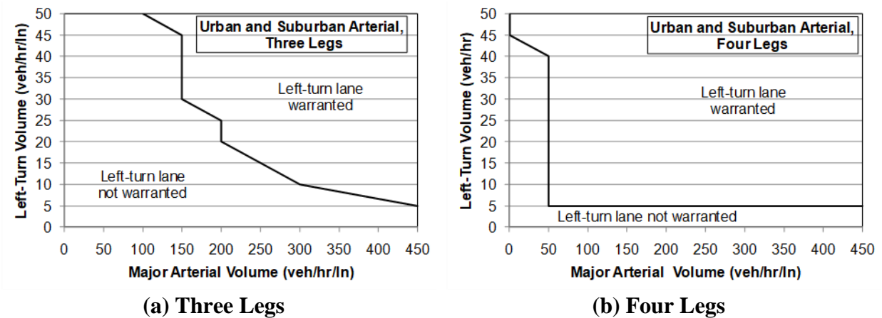
Figure 19. Suggested Left-Turn Lane Warrants Based on Results from Benefit-Cost Evaluations for Intersections on Urban and Suburban Arterials (6I)
